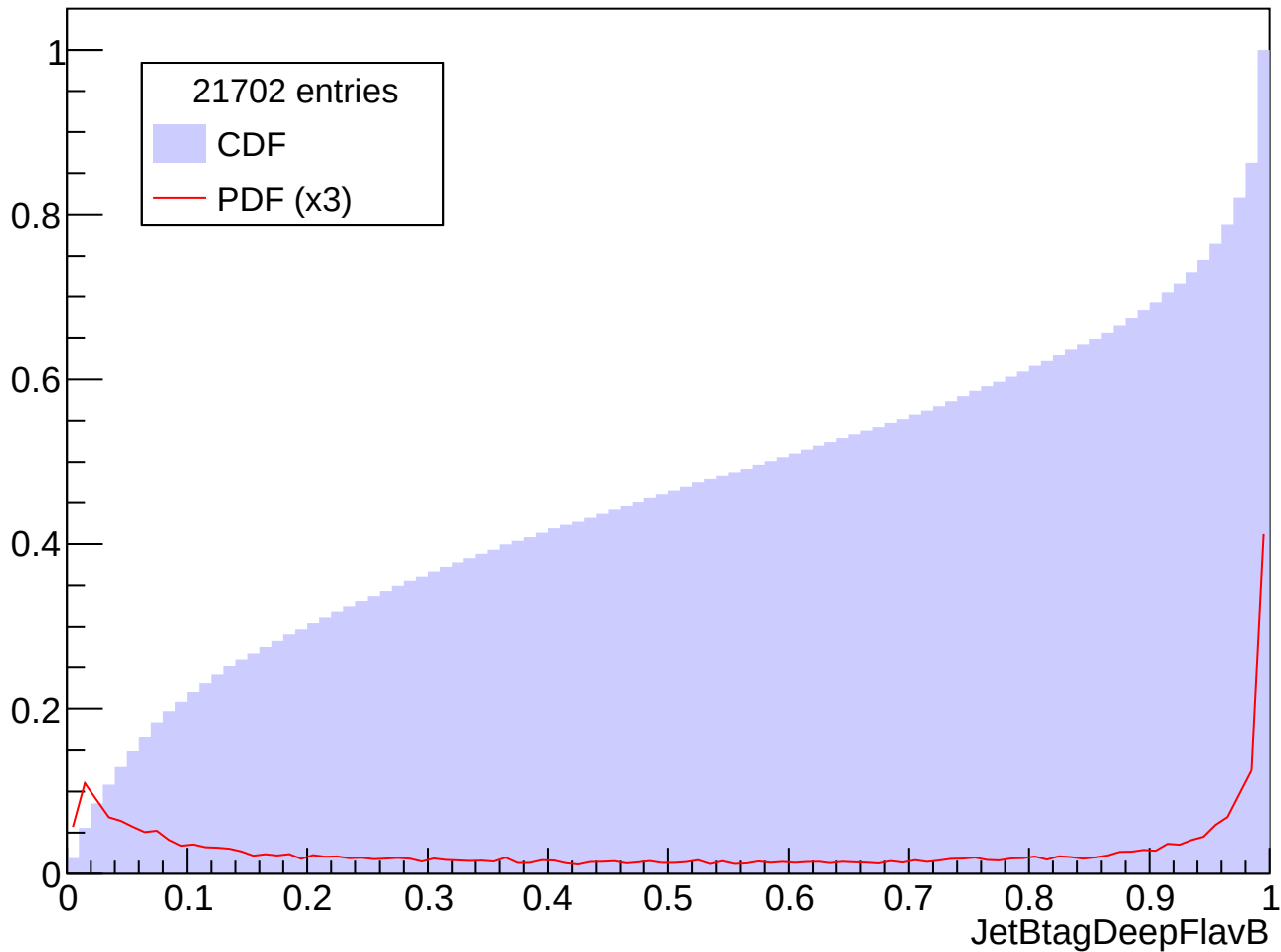
Prob. Distrib. for abs(Eta) in [2.0, 2.5], Pt in [160, 180] GeV
