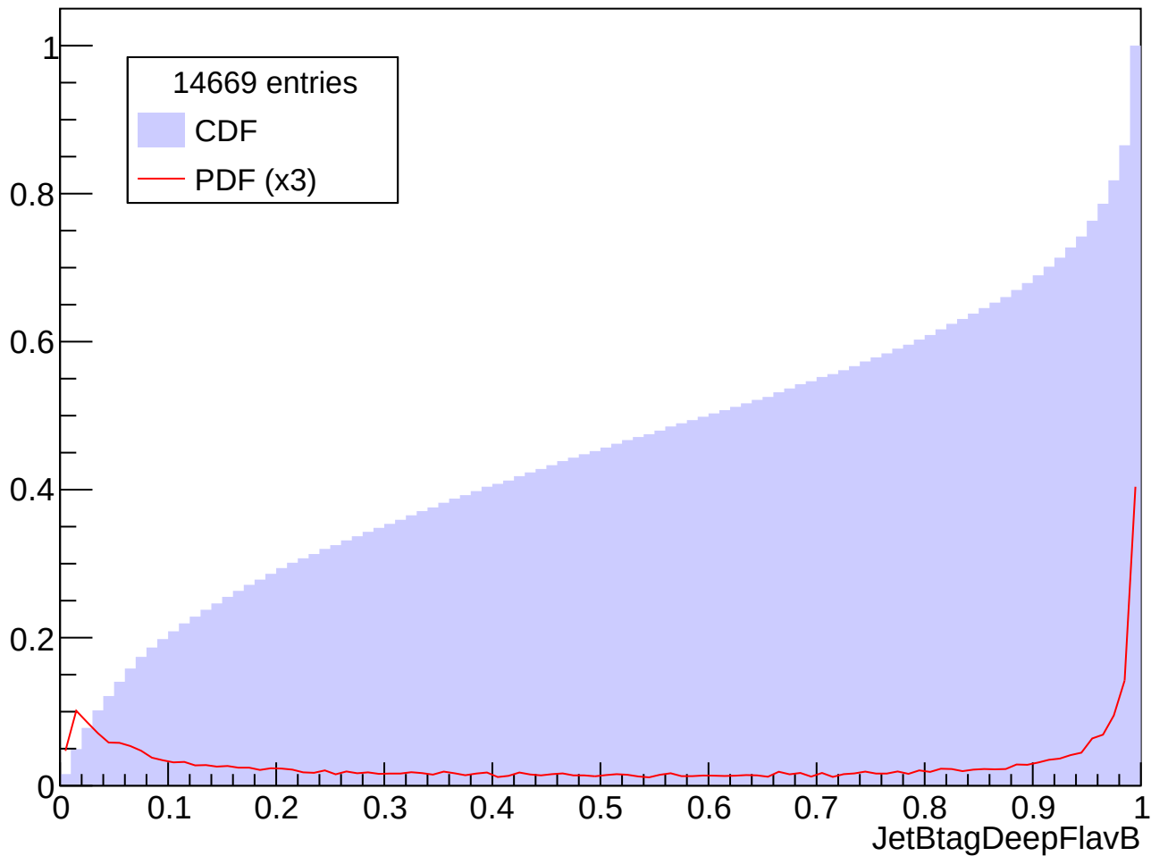
Prob. Distrib. for abs(Eta) in [2.0, 2.5], Pt in [180, 200] GeV
