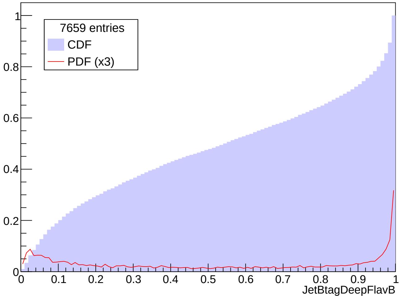
Prob. Distrib. for abs(Eta) in [2.0, 2.5], Pt in [250, 300] GeV
