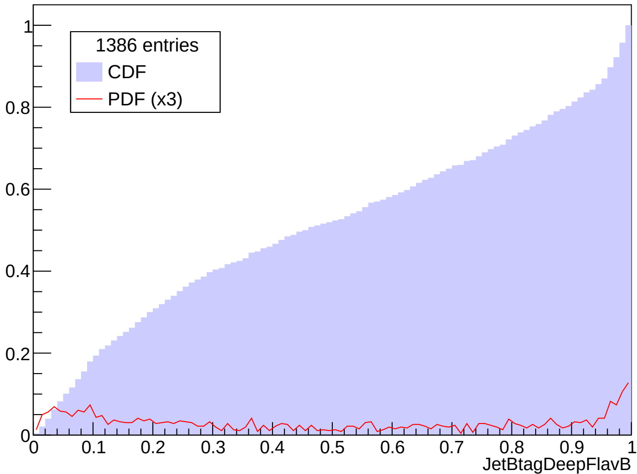
Prob. Distrib. for abs(Eta) in [2.0, 2.5], Pt in [400, 600] GeV
