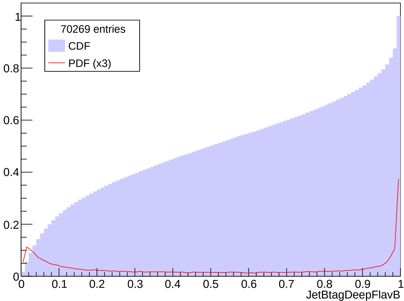
Prob. Distrib. for abs(Eta) in [2.0, 2.5], Pt in [50, 60] GeV
