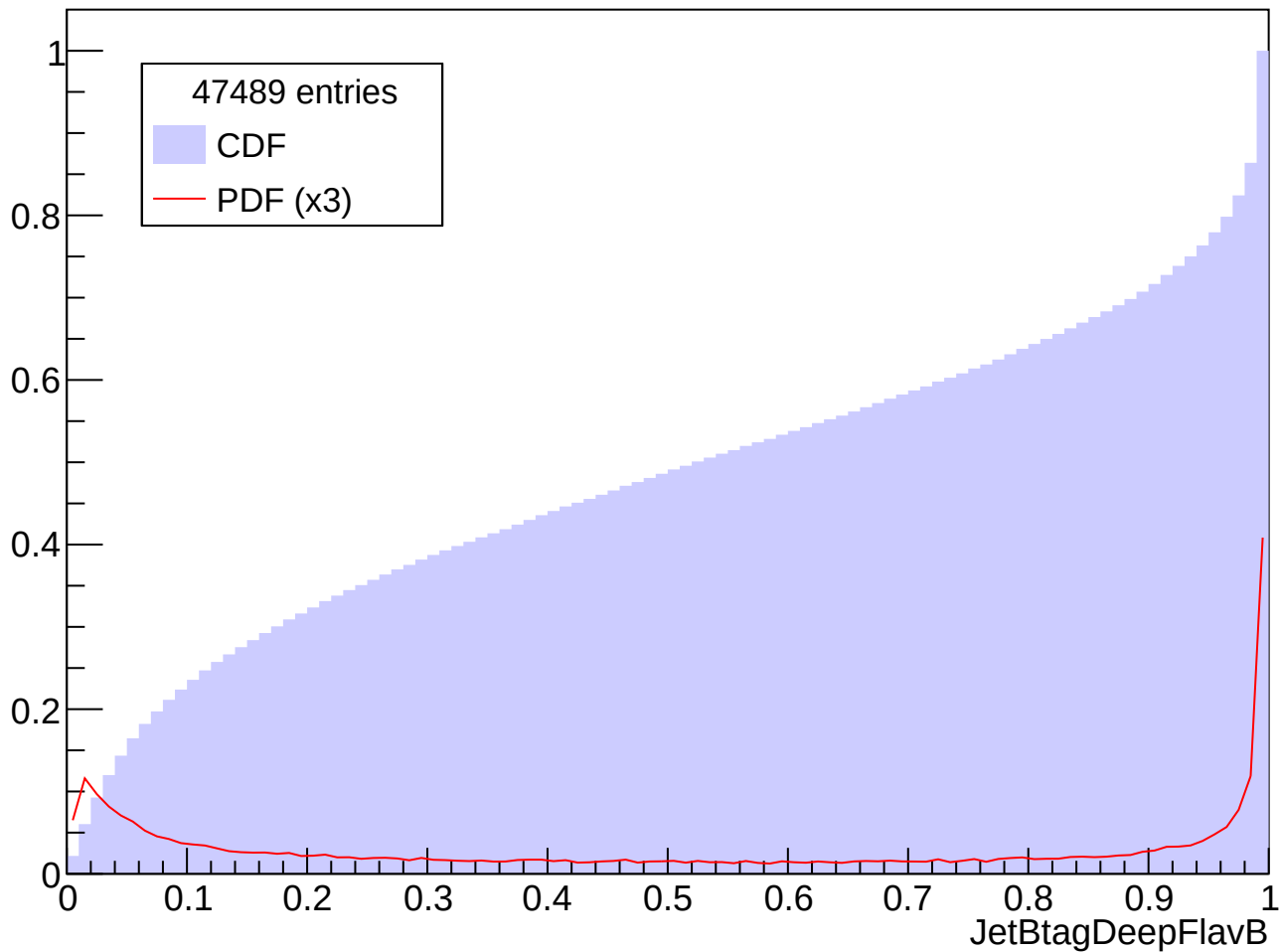
Prob. Distrib. for abs(Eta) in [2.0, 2.5], Pt in [70, 80] GeV
