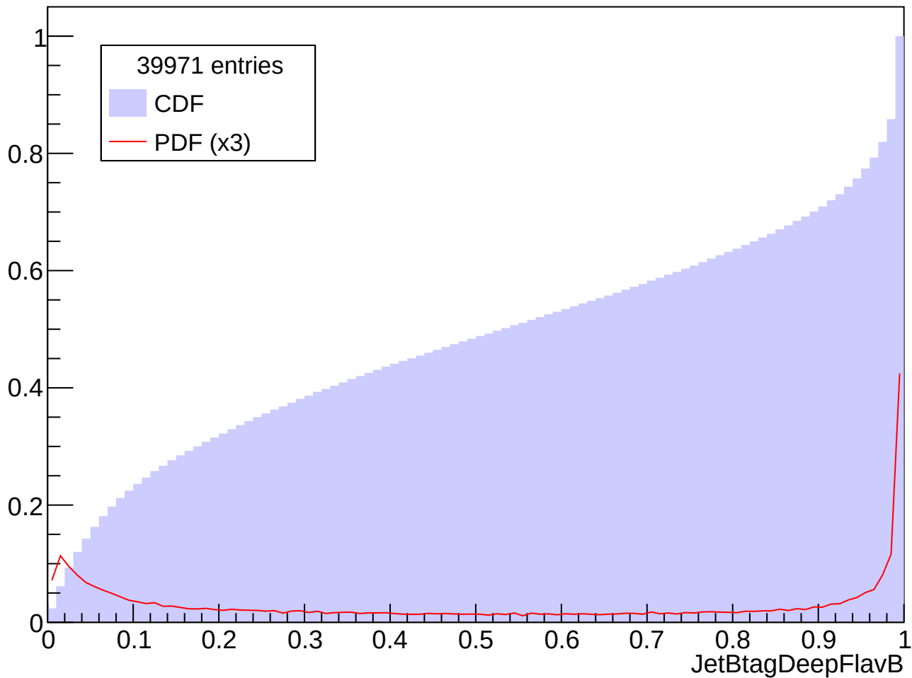
Prob. Distrib. for abs(Eta) in [2.0, 2.5], Pt in [80, 90] GeV
