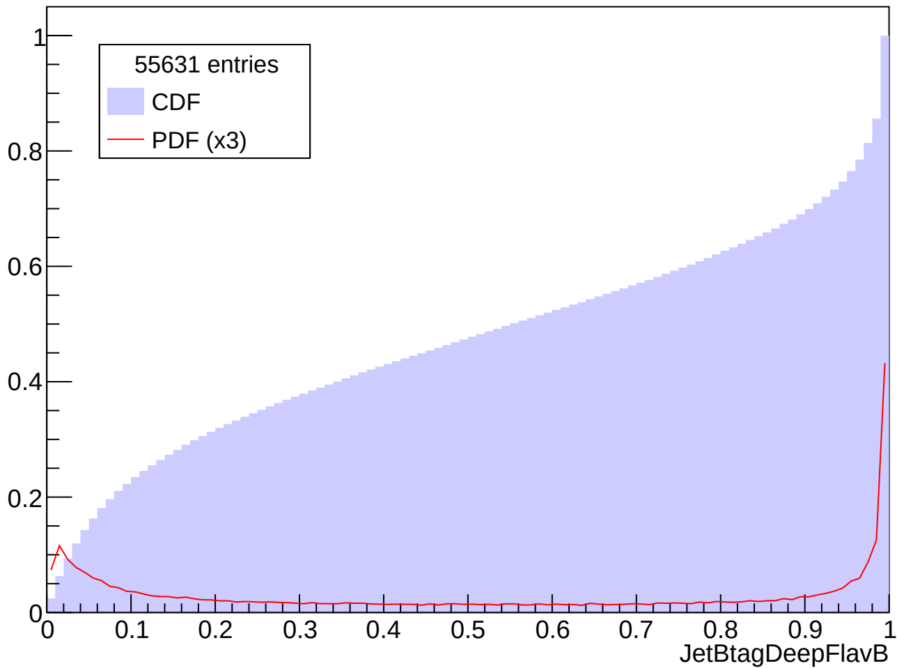
Prob. Distrib. for abs(Eta) in [2.0, 2.5], Pt in [100, 120] GeV
