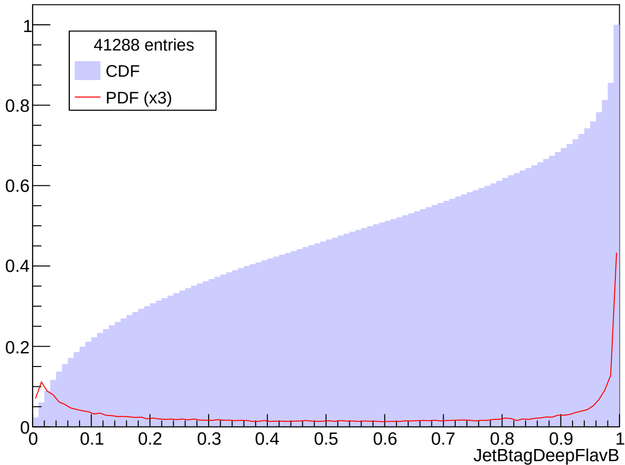
Prob. Distrib. for abs(Eta) in [2.0, 2.5], Pt in [120, 140] GeV
