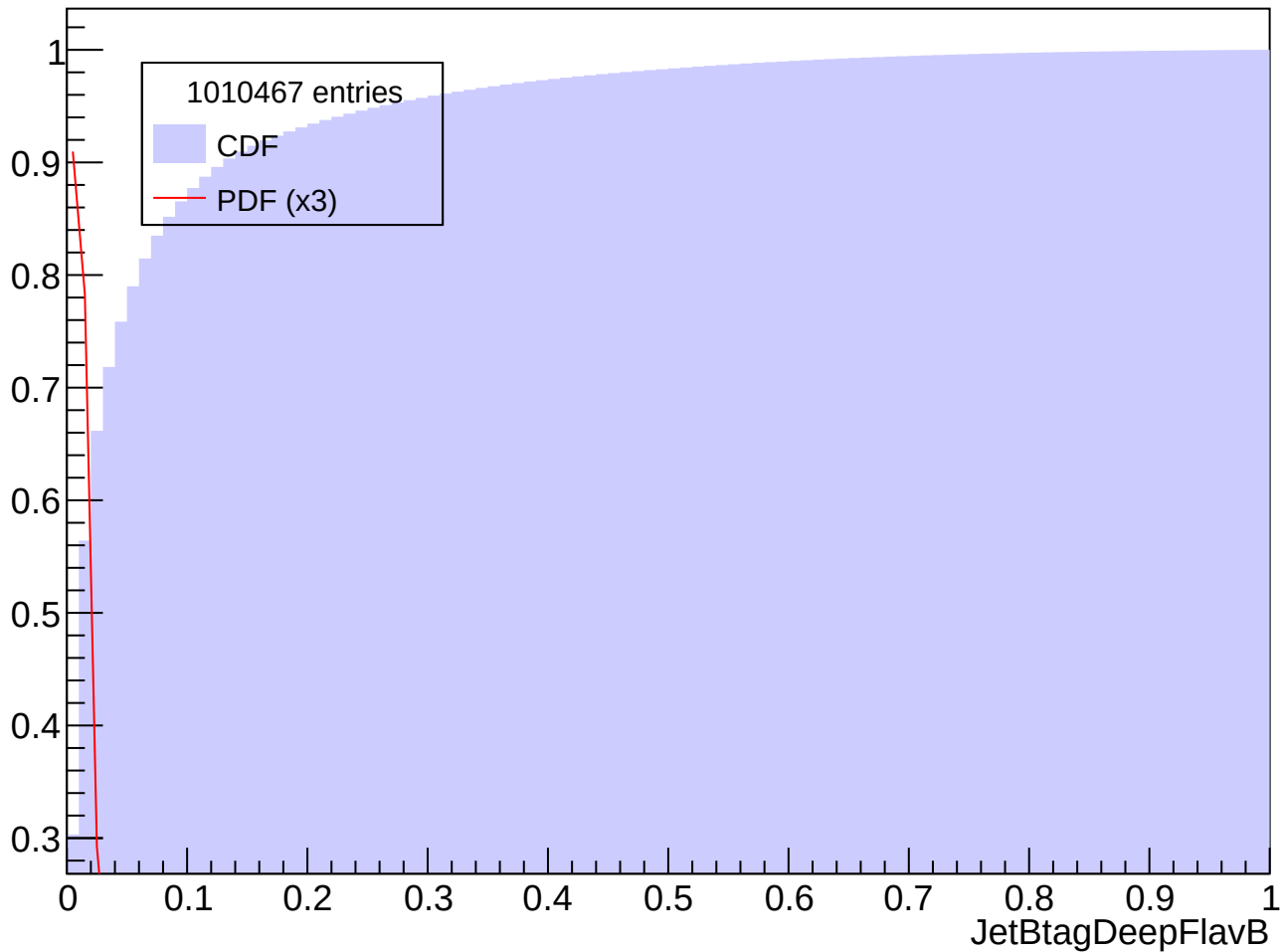
Prob. Distrib. for abs(Eta) in [0.0, 0.5], Pt in [30, 40] GeV
