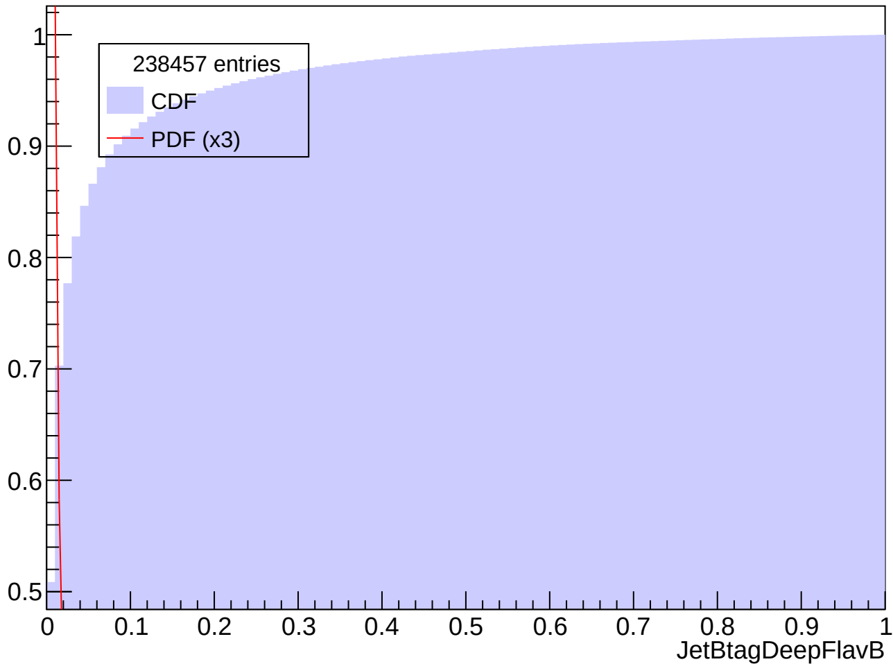
Prob. Distrib. for abs(Eta) in [0.0, 0.5], Pt in [160, 180] GeV
