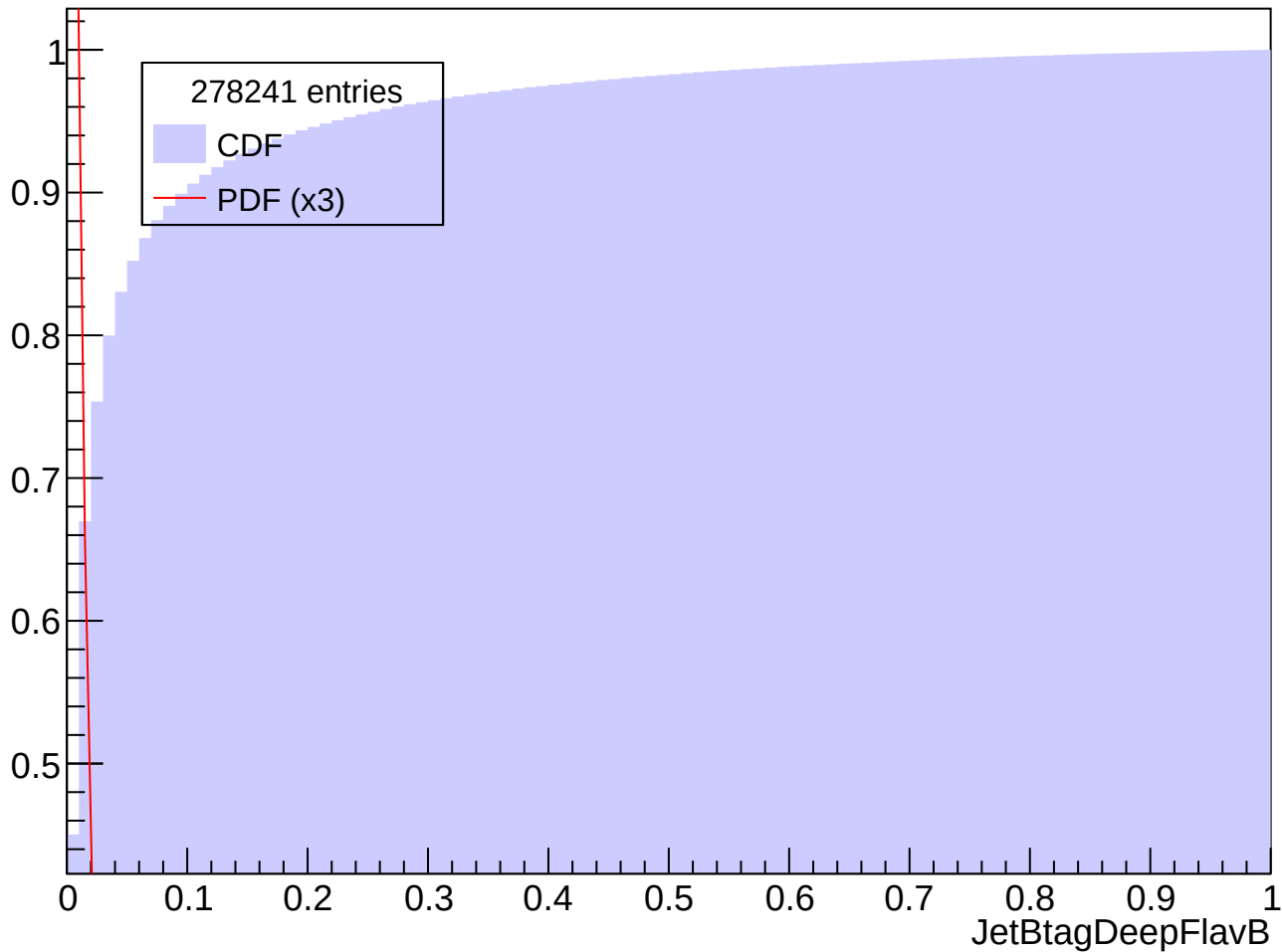
Prob. Distrib. for abs(Eta) in [0.0, 0.5], Pt in [200, 250] GeV
