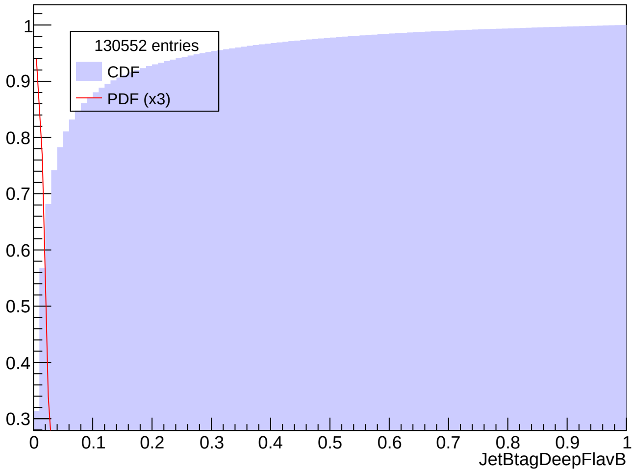
Prob. Distrib. for abs(Eta) in [0.0, 0.5], Pt in [300, 400] GeV
