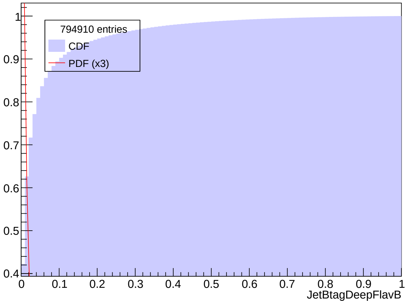
Prob. Distrib. for abs(Eta) in [0.0, 0.5], Pt in [40, 50] GeV
