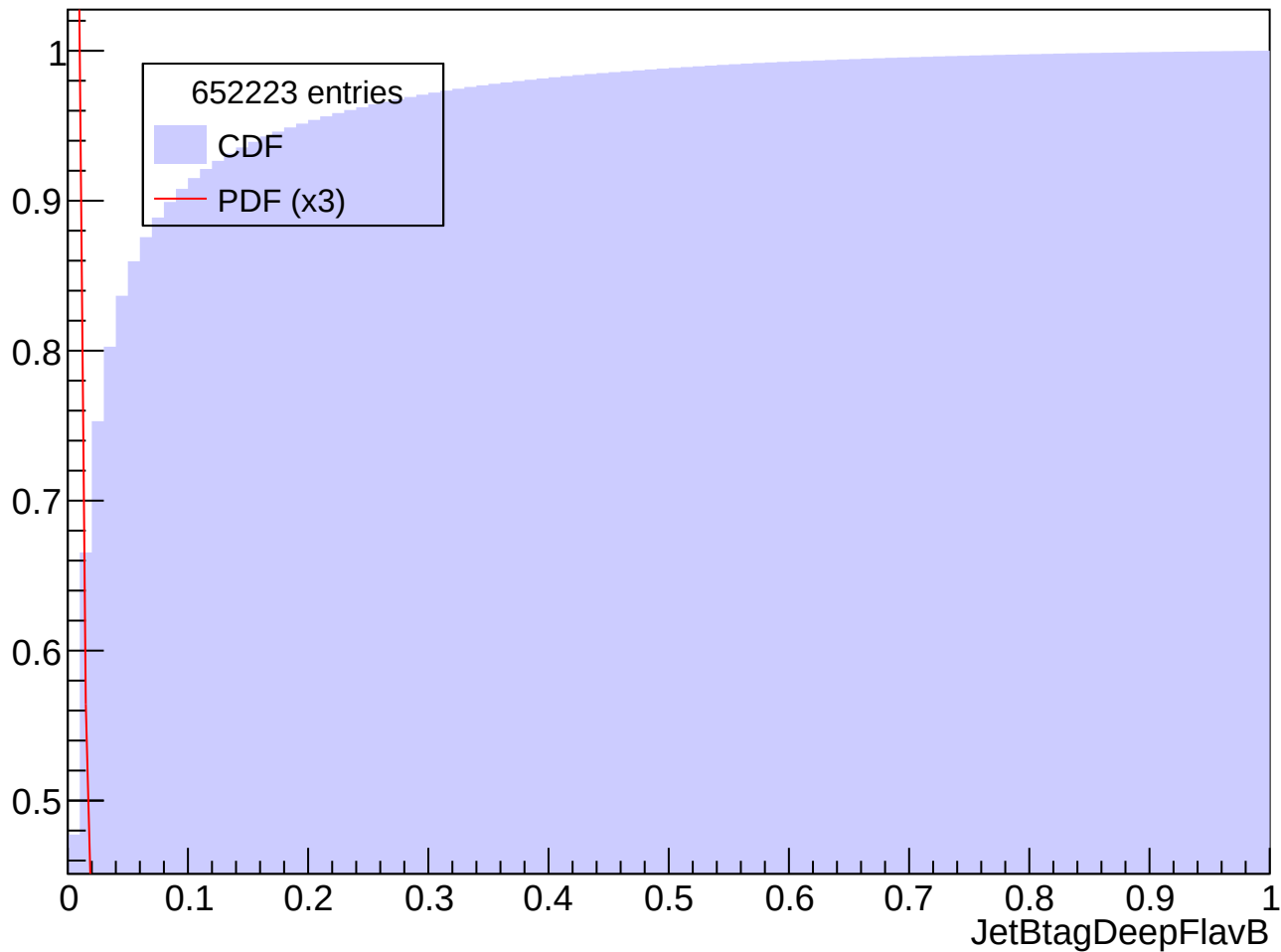
Prob. Distrib. for abs(Eta) in [0.0, 0.5], Pt in [50, 60] GeV
