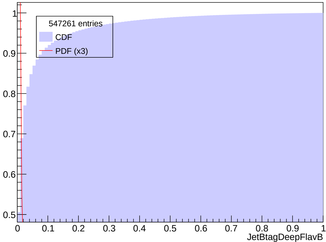
Prob. Distrib. for abs(Eta) in [0.0, 0.5], Pt in [60, 70] GeV
