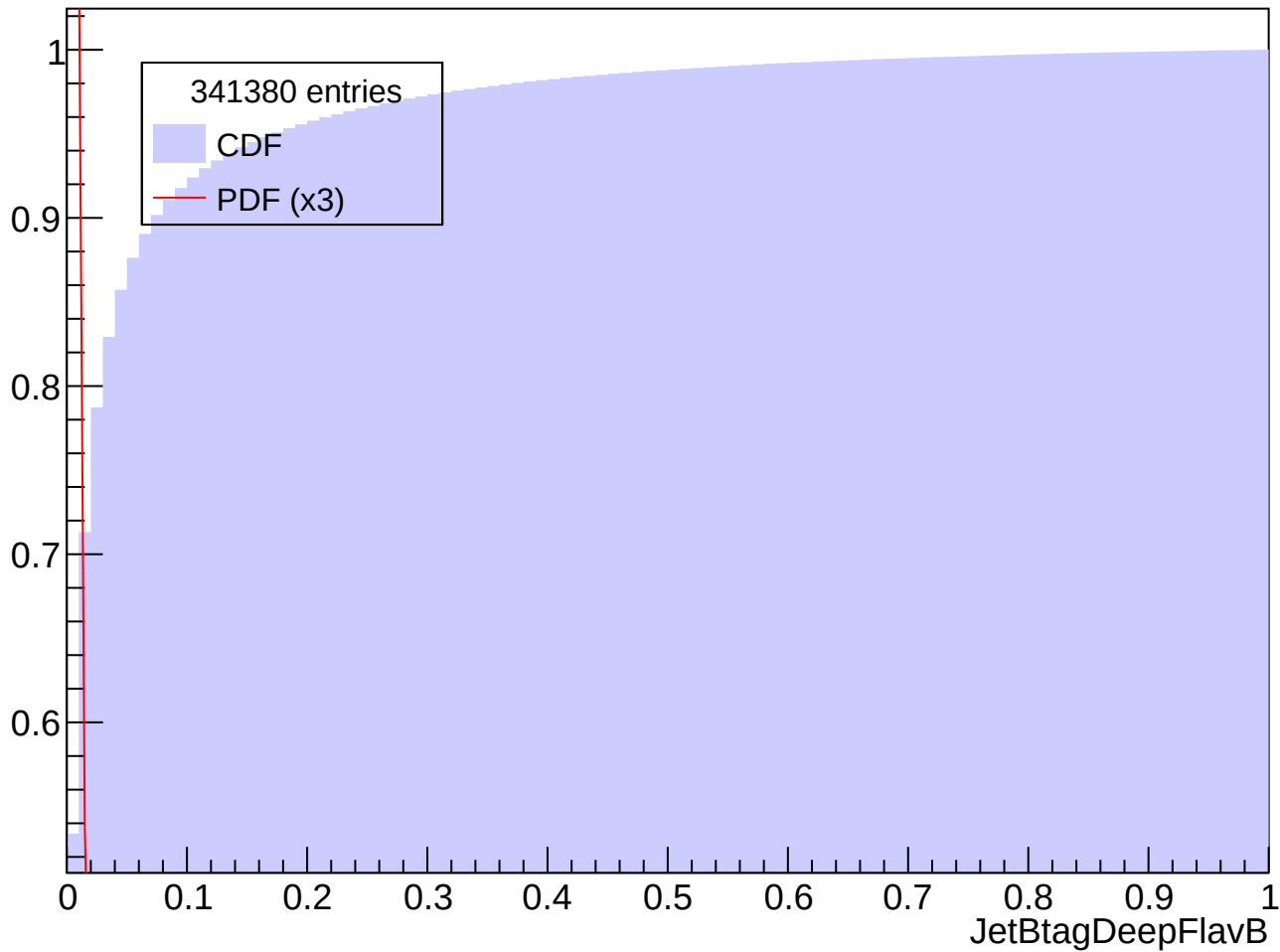
Prob. Distrib. for abs(Eta) in [0.0, 0.5], Pt in [90, 100] GeV
