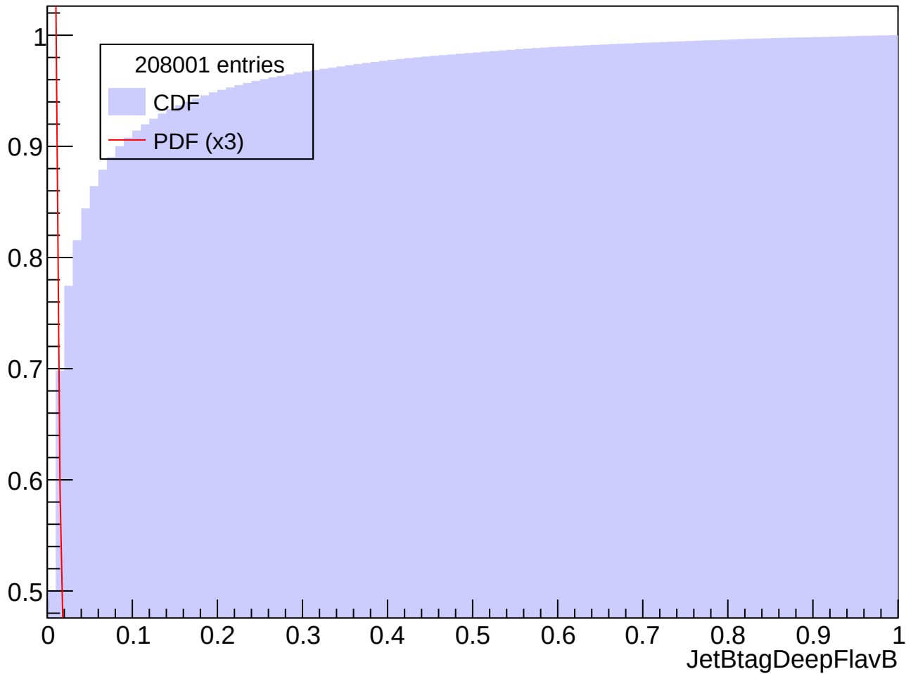
Prob. Distrib. for abs(Eta) in [0.5, 1.0], Pt in [160, 180] GeV
