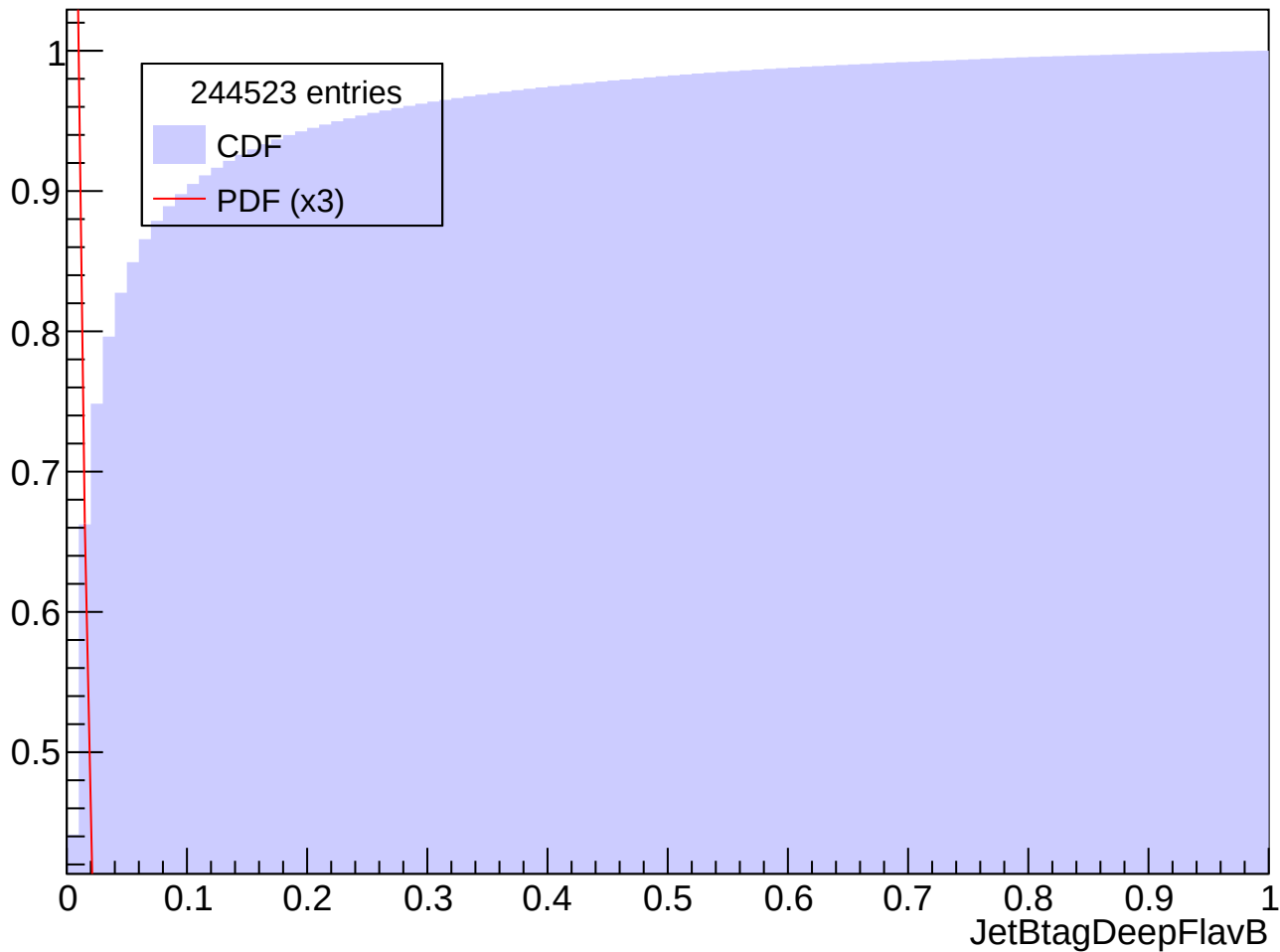
Prob. Distrib. for abs(Eta) in [0.5, 1.0], Pt in [200, 250] GeV
