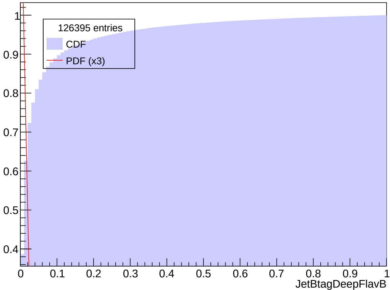
Prob. Distrib. for abs(Eta) in [0.5, 1.0], Pt in [250, 300] GeV
