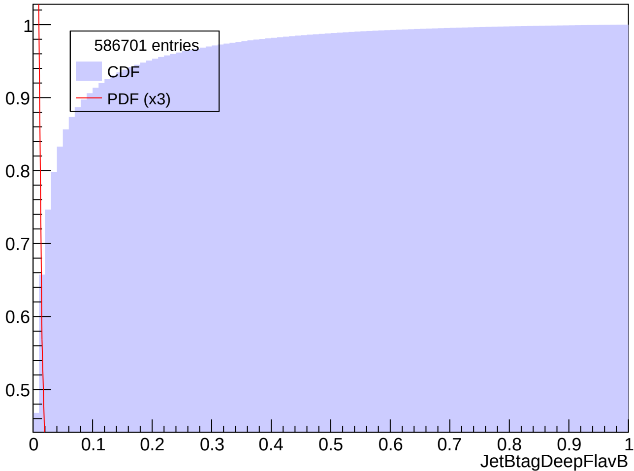
Prob. Distrib. for abs(Eta) in [0.5, 1.0], Pt in [50, 60] GeV
