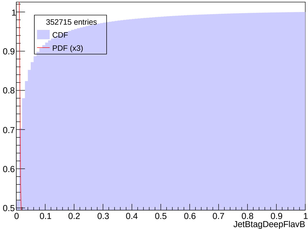
Prob. Distrib. for abs(Eta) in [0.5, 1.0], Pt in [80, 90] GeV
