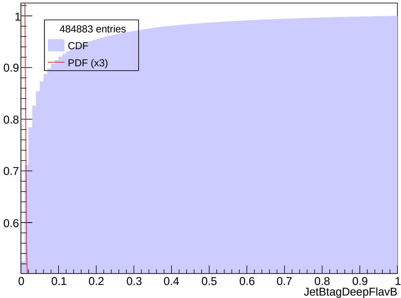
Prob. Distrib. for abs(Eta) in [0.5, 1.0], Pt in [100, 120] GeV
