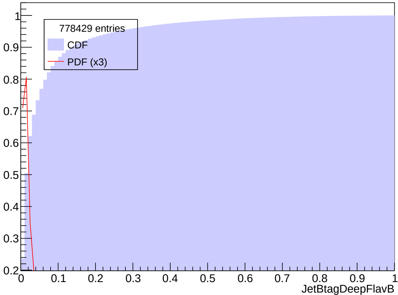
Prob. Distrib. for abs(Eta) in [1.0, 1.5], Pt in [30, 40] GeV
