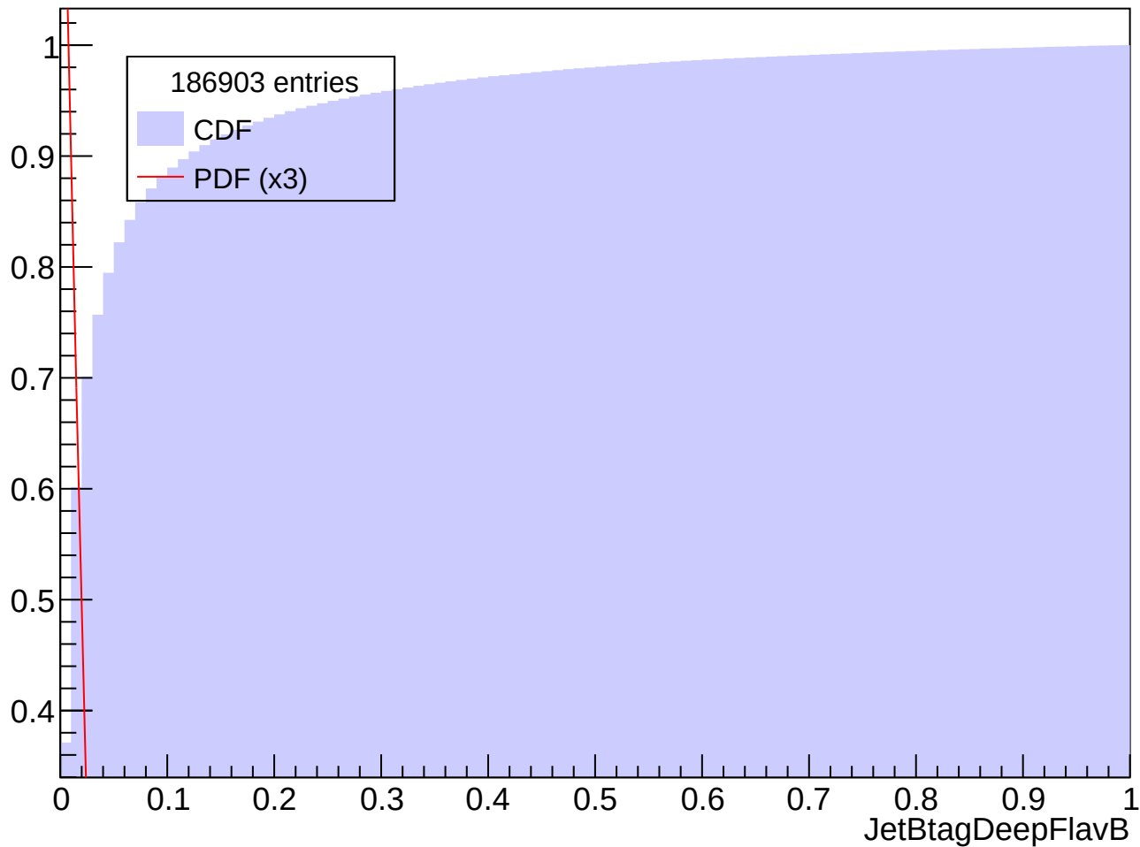
Prob. Distrib. for abs(Eta) in [1.0, 1.5], Pt in [200, 250] GeV
