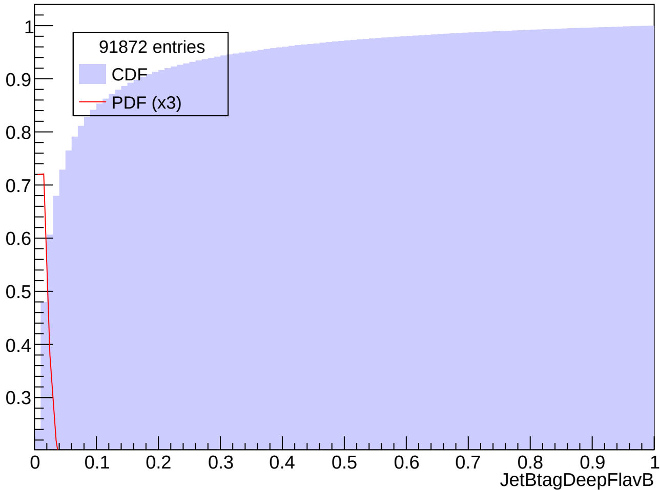
Prob. Distrib. for abs(Eta) in [1.0, 1.5], Pt in [300, 400] GeV
