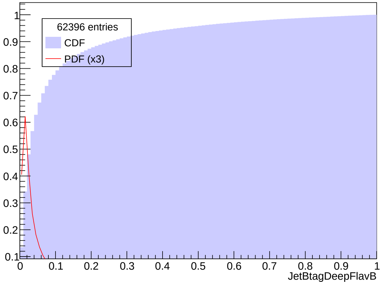
Prob. Distrib. for abs(Eta) in [1.0, 1.5], Pt in [400, 600] GeV
