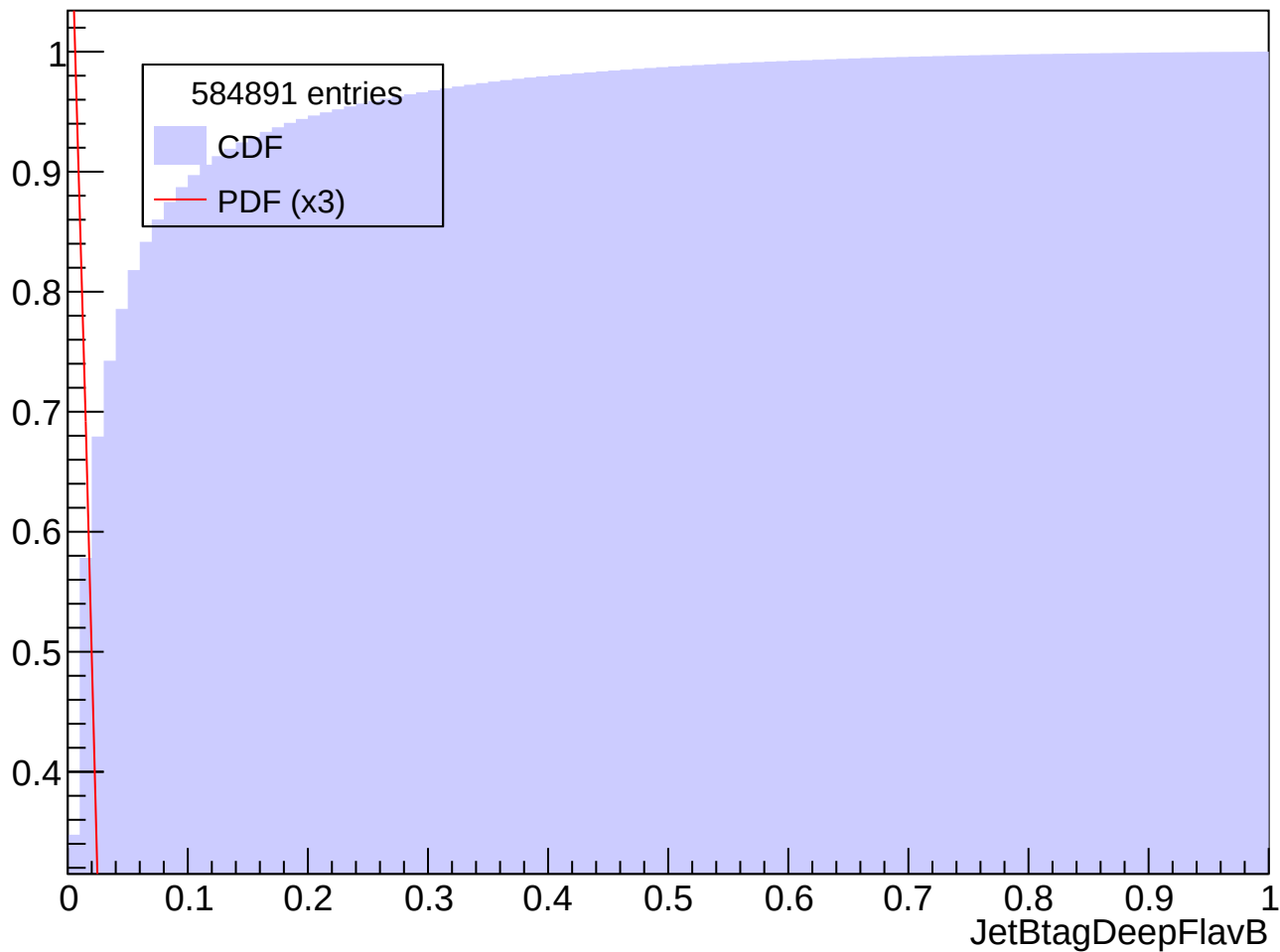
Prob. Distrib. for abs(Eta) in [1.0, 1.5], Pt in [40, 50] GeV
