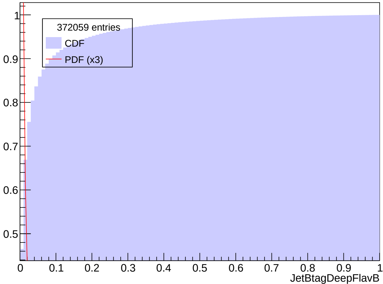
Prob. Distrib. for abs(Eta) in [1.0, 1.5], Pt in [100, 120] GeV
