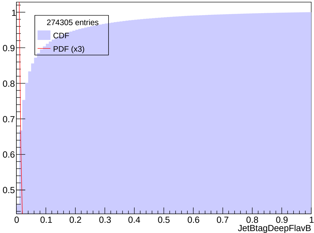
Prob. Distrib. for abs(Eta) in [1.0, 1.5], Pt in [120, 140] GeV
