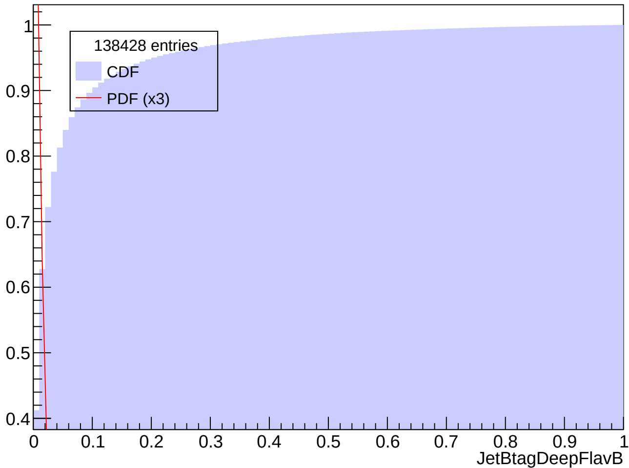
Prob. Distrib. for abs(Eta) in [1.5, 2.0], Pt in [140, 160] GeV
