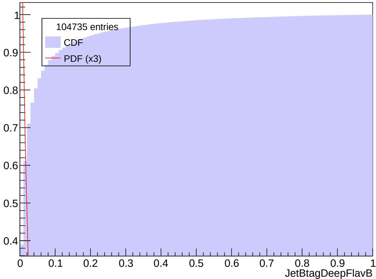
Prob. Distrib. for abs(Eta) in [1.5, 2.0], Pt in [160, 180] GeV
