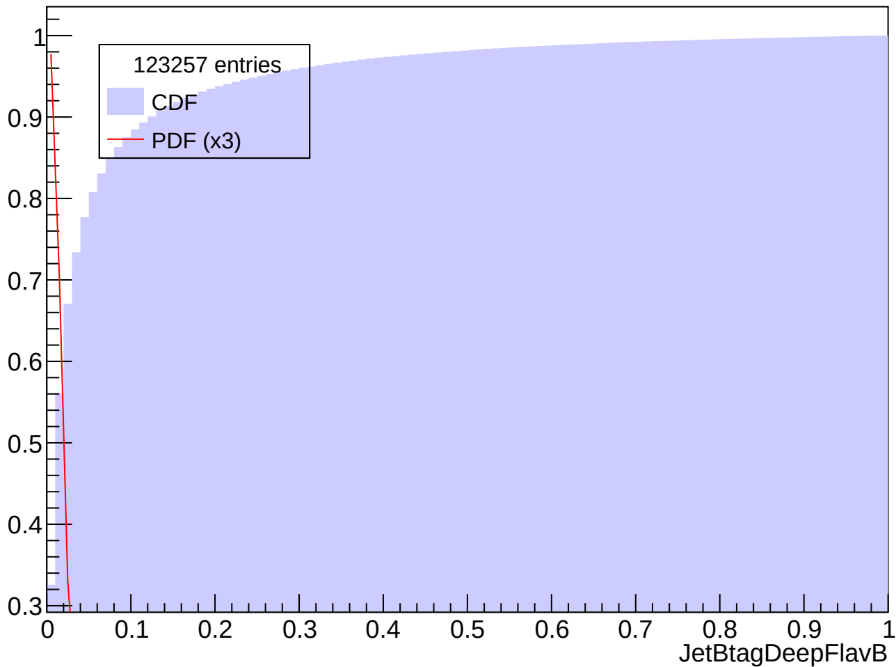
Prob. Distrib. for abs(Eta) in [1.5, 2.0], Pt in [200, 250] GeV
