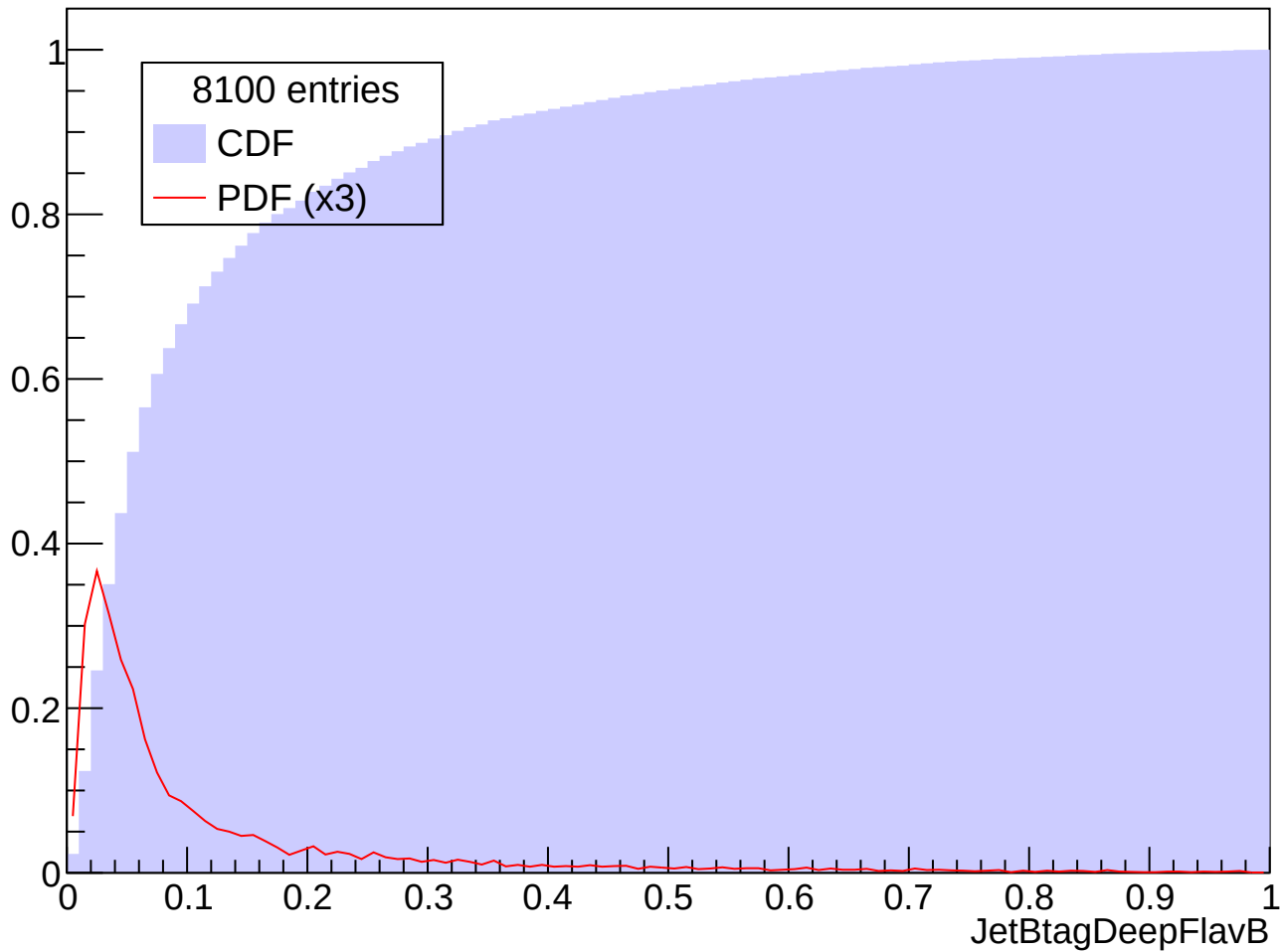
Prob. Distrib. for abs(Eta) in [1.5, 2.0], Pt in [600, 1000] GeV
