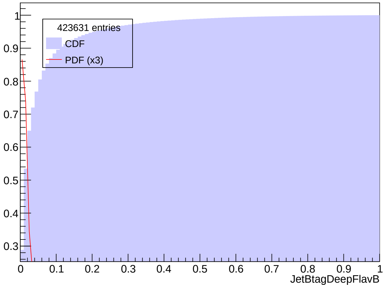
Prob. Distrib. for abs(Eta) in [1.5, 2.0], Pt in [40, 50] GeV
