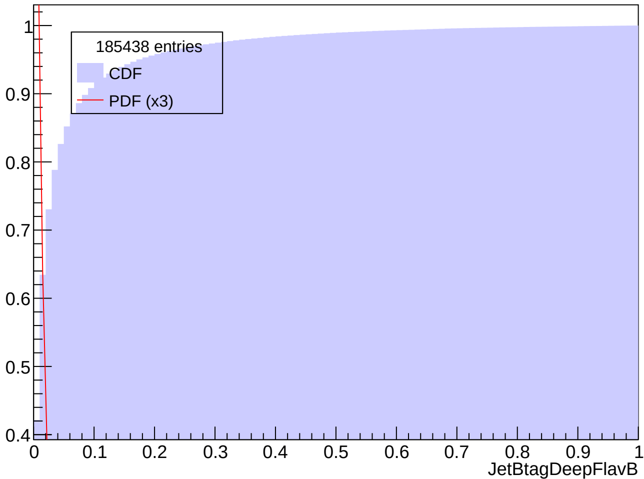
Prob. Distrib. for abs(Eta) in [1.5, 2.0], Pt in [80, 90] GeV
