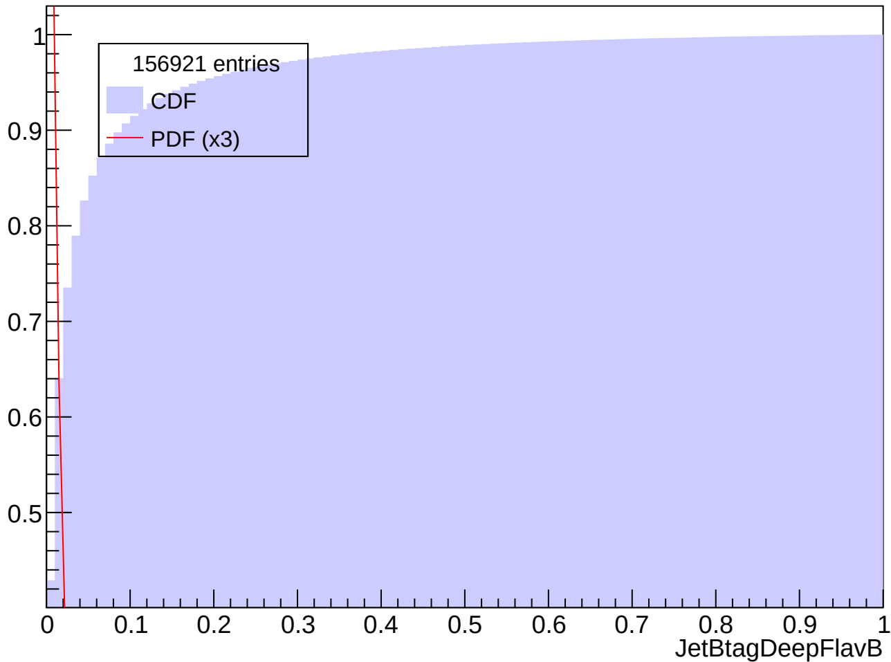
Prob. Distrib. for abs(Eta) in [1.5, 2.0], Pt in [90, 100] GeV
