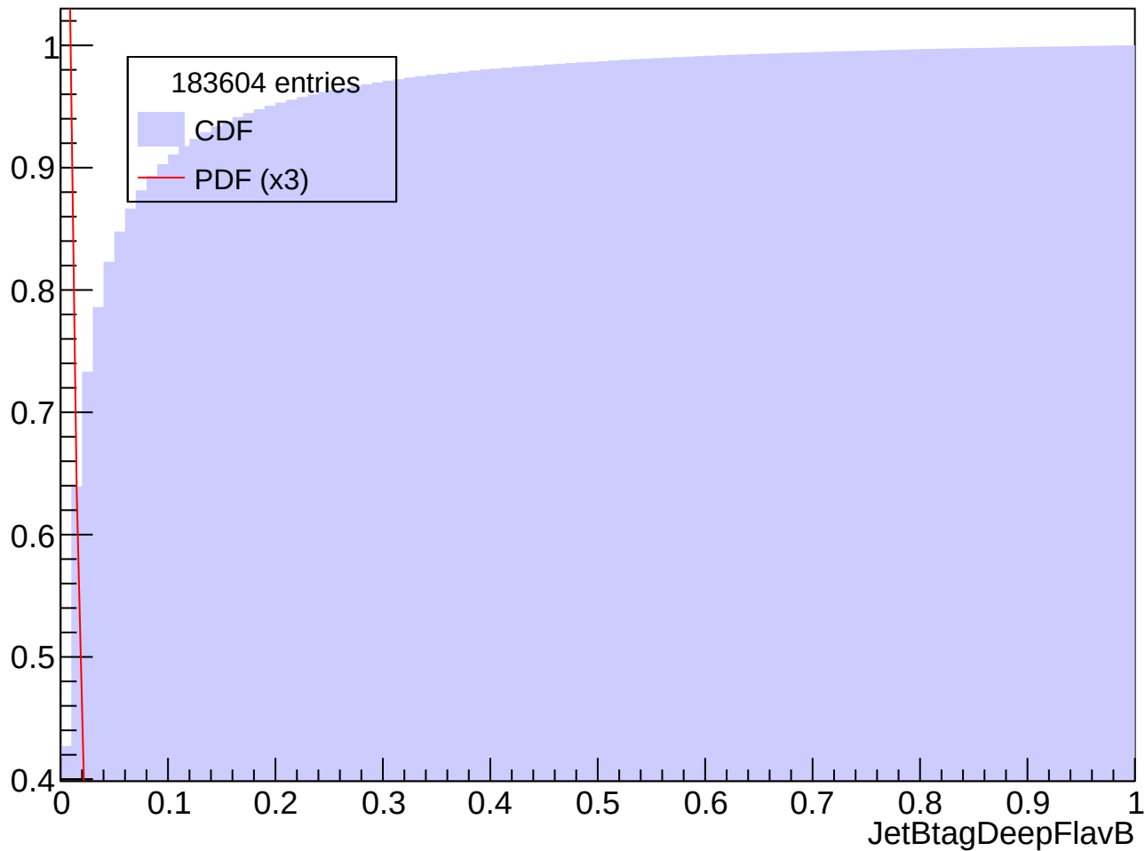
Prob. Distrib. for abs(Eta) in [1.5, 2.0], Pt in [120, 140] GeV
