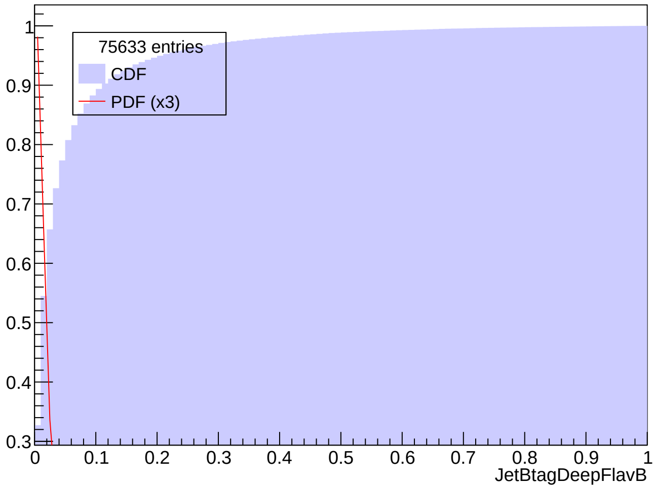
Prob. Distrib. for abs(Eta) in [2.0, 2.5], Pt in [140, 160] GeV
