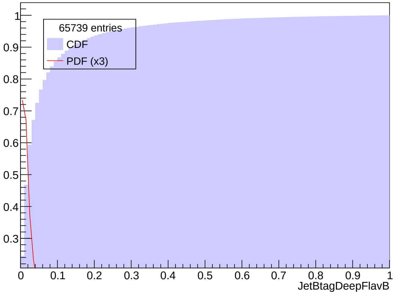
Prob. Distrib. for abs(Eta) in [2.0, 2.5], Pt in [200, 250] GeV
