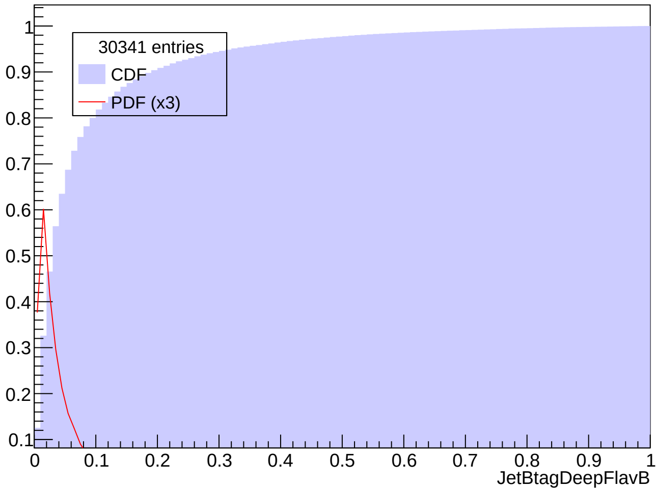
Prob. Distrib. for abs(Eta) in [2.0, 2.5], Pt in [300, 400] GeV
