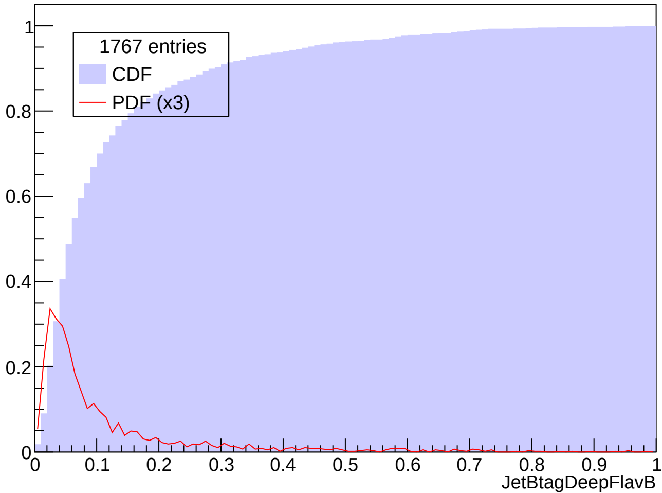
Prob. Distrib. for abs(Eta) in [2.0, 2.5], Pt in [600, 1000] GeV
