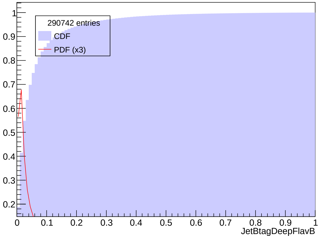
Prob. Distrib. for abs(Eta) in [2.0, 2.5], Pt in [40, 50] GeV
