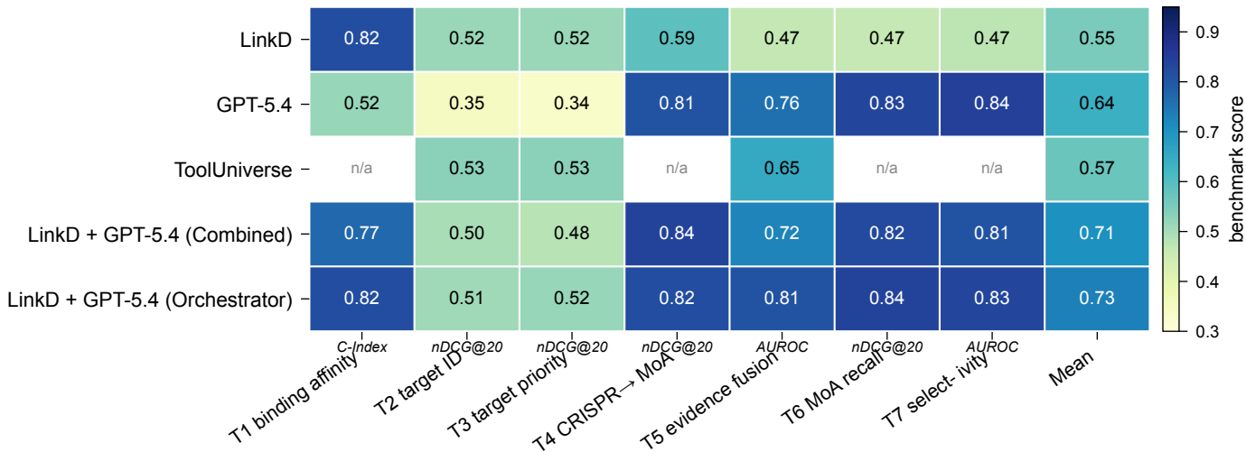
LinkD vs GPT-5.4 vs ToolUniverse vs LinkD+GPT-5.4 across drug-discovery tasks
