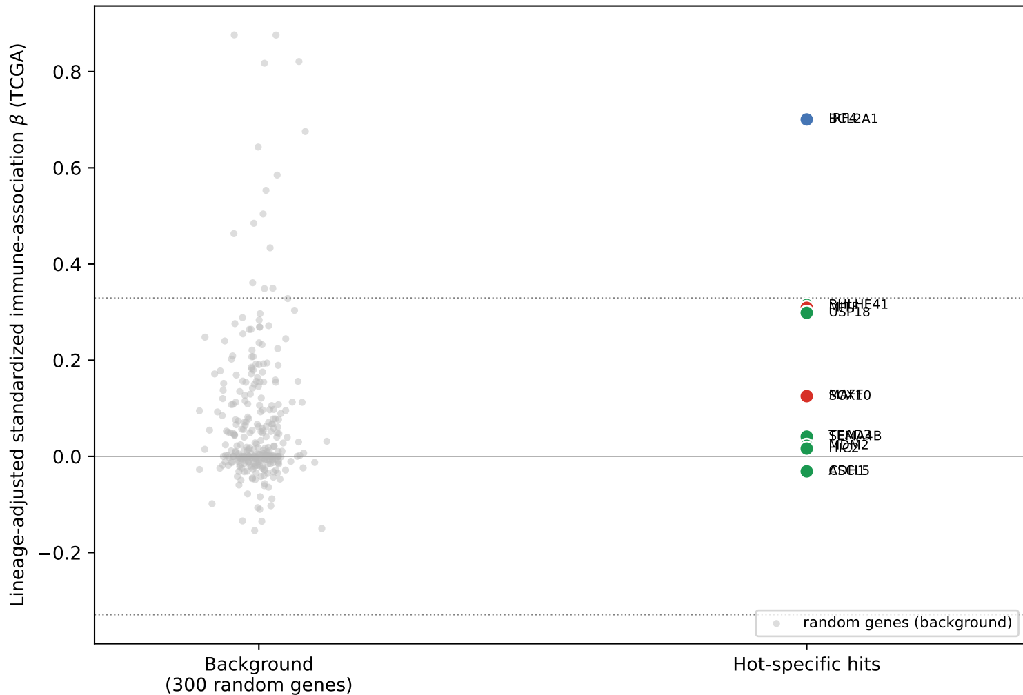
Real-TME corroborator (TCGA, n=10{,}534 tumors) Effect size of immune association after lineage adjustment red=melanocyte-lineage; green=tumor-intrinsic (within background); blue=immune-associated
