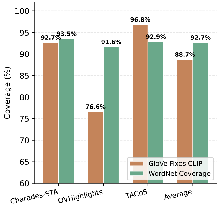
GloVe & WordNet Complementary Coverage
