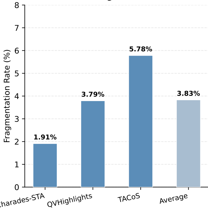
CLIP BPE Fragmentation Rate
