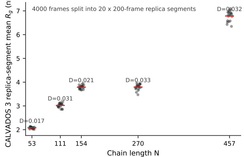
D CALVADOS 3 merged 20-replica trajectories
