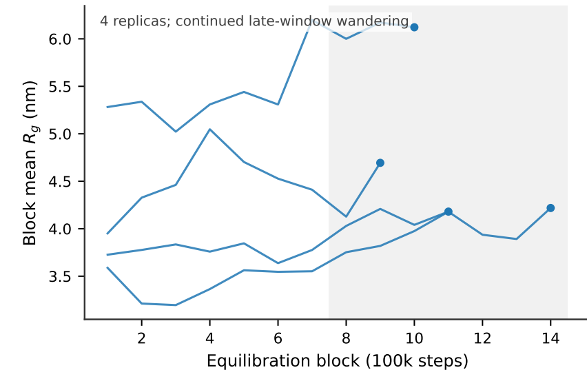
C Mpipi slow-mixing example (N=457)
