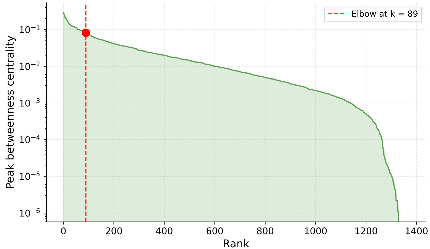
Betweenness centrality ranking (n = 1368)
