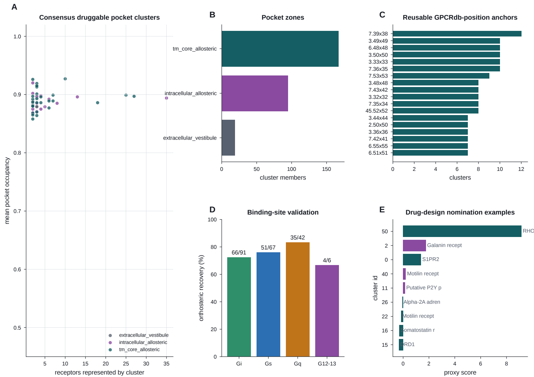
Figure 6 candidate: drug-design pocket atlas
