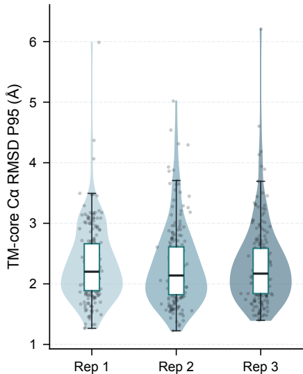
A Receptor TM-core displacement
