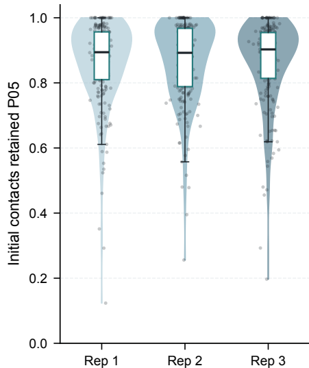
C Interface-contact retention
