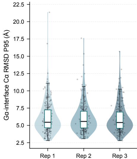
B Gα interface-region displacement
